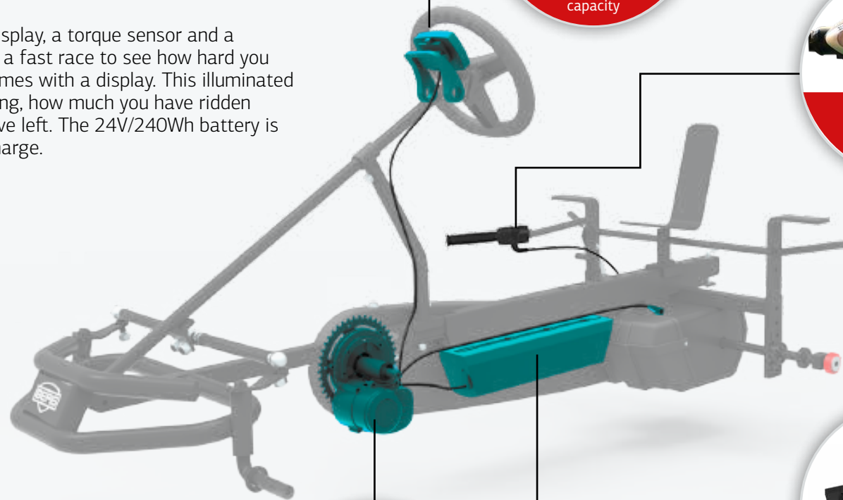
BFR-3 Three gears
